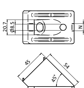
Winkelverbinder 45, 45° Angle Connector 45, 45°
