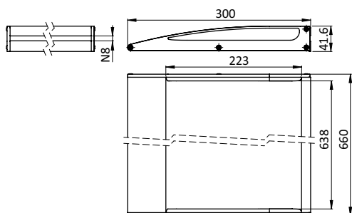
Keyboard Holder AL, Slot 8 Tastaturhalter AL, Nut 8
