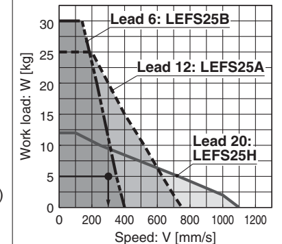
<Speed-Work load graph> (LEFS25/Step motor)
