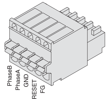
Counter plug
