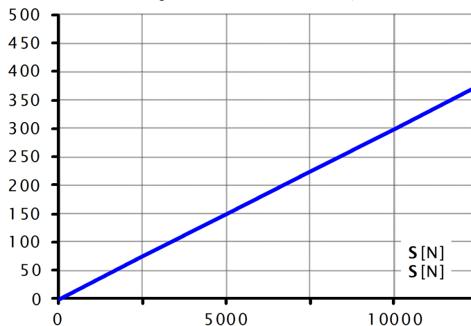
F [N] Diagramma Spinta S - Forza F ; L=500 mm Diagram Force S - Force F ; L=500mm
