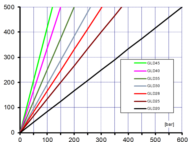
Diagramma Pressione-Forza; L=1000mm Diagram Pressure-Force; L=1000mm
