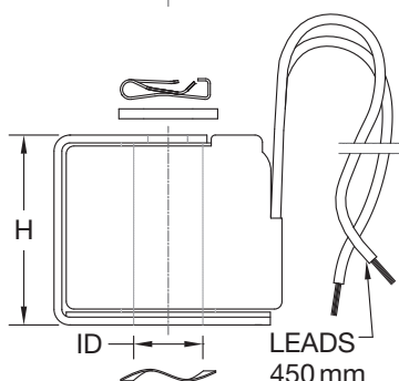
BF COIL LEADS 450mm [18"]
