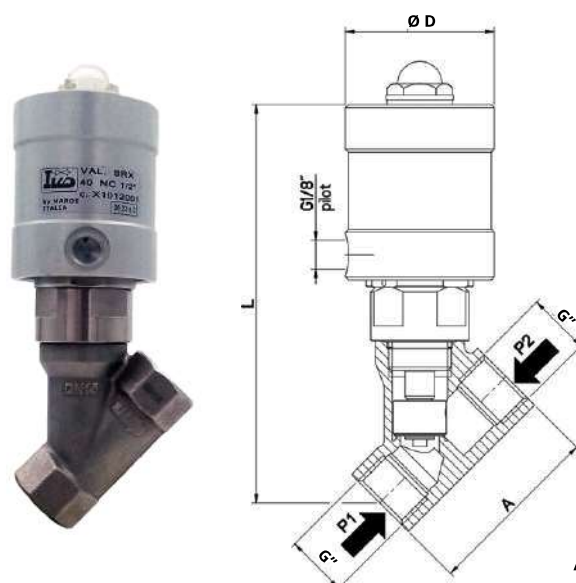
SRX - NC Closing against flow / SRX - NC Ingresso fluido sotto otturatore
