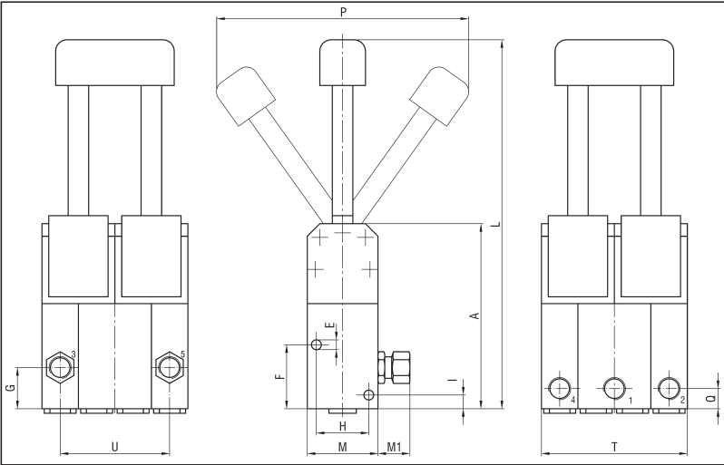
5/3 C.C. MANOPOLA VERTICALE G 1/8
