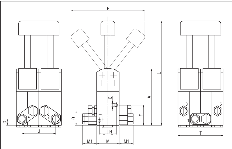
5/3 C.C. MANOPOLA VERTICALE G 1/4 - G 1/2
