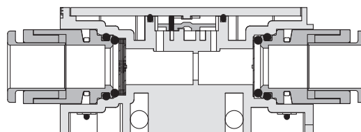
PF2M711-C8(-L)
